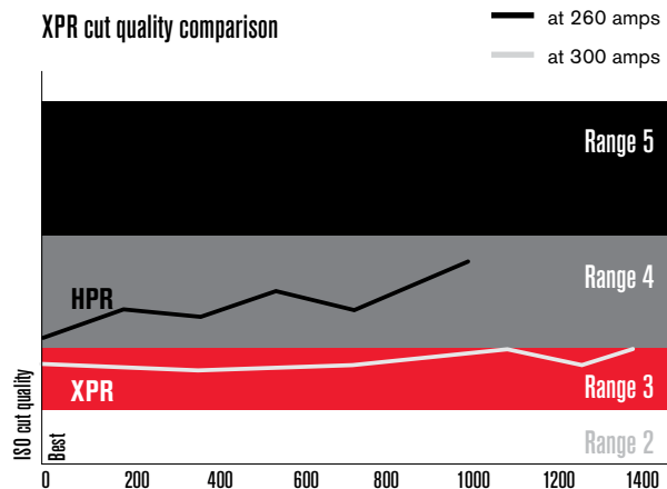
20-second cuts on mild steel
